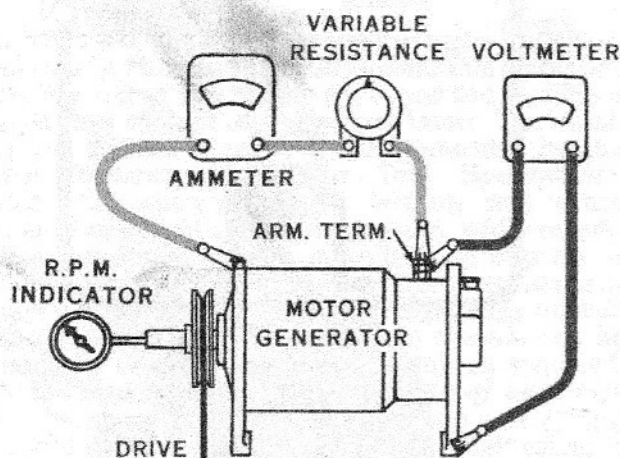
Figure 7—Checking motor-generator output.
